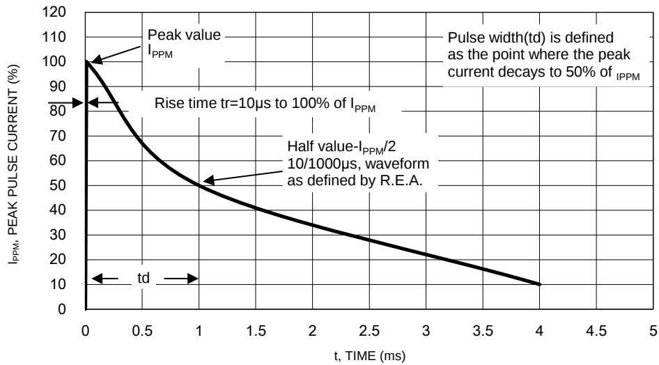
Fig.8 Pulse Waveform
