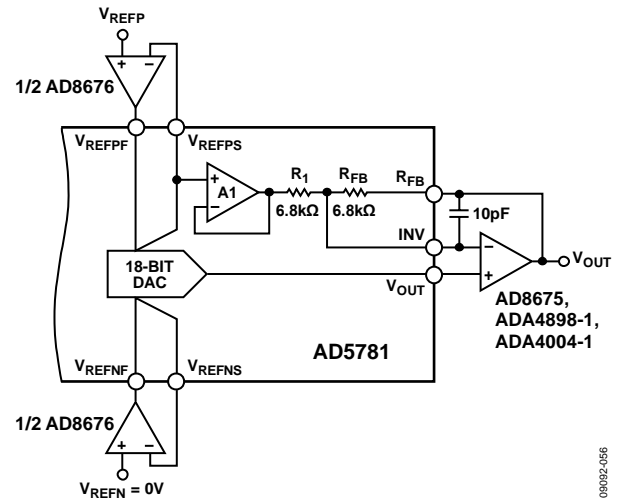
Figure 53. Output Amplifier in Gain of Two Configuration
