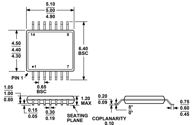
COMPLIANT TO JEDEC STANDARDS MO-153-AB-1 Figure 60. 14-Lead Thin Shrink Small Outline Package [TSSOP] (RU-14) Dimensions shown in millimeters
