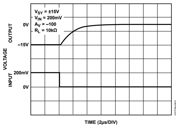
Figure 42. Positive Overload Recovery
