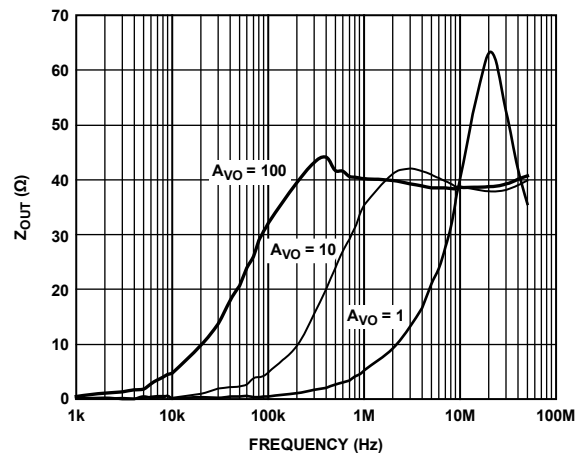
Figure 14. Z_{OUT} vs. Frequency
