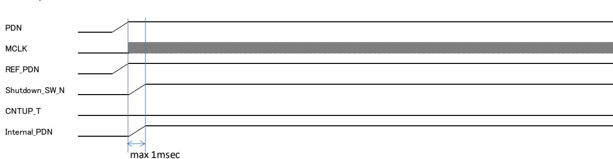
Figure 60. Internal PDN Release Sequence
