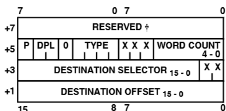
FIGURE 11. GATE DESCRIPTOR
