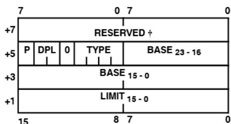
FIGURE 10. SYSTEM SEGMENT DESCRIPTOR
