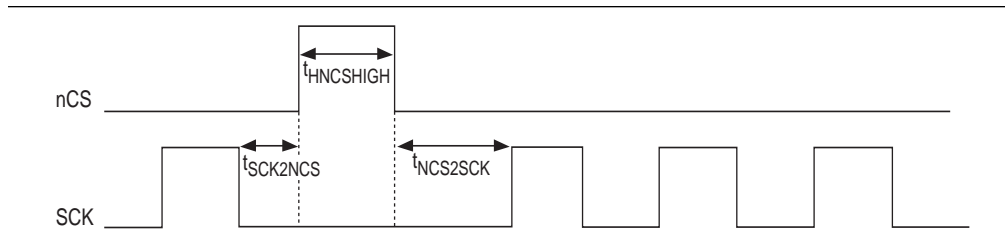
Figure 9–37. SPI Timing Waveform
