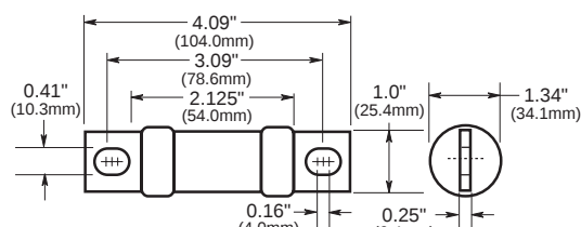
125-200 Ampere Rating
