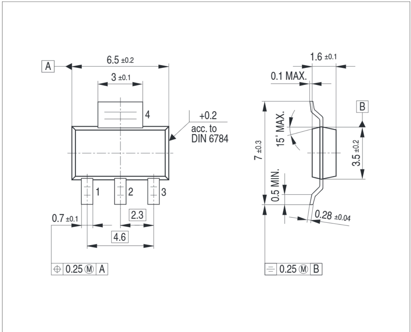
Figure 6 PG-SOT223-4
