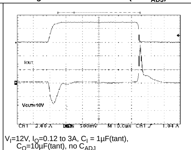
Figure 23. Load transient (No C_{\text{ADJ}} )
