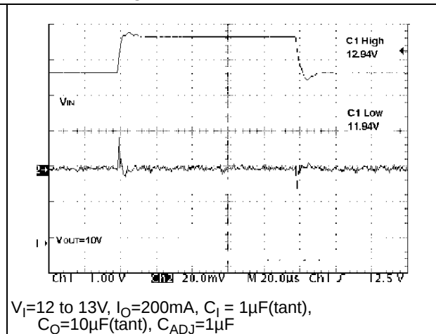
Figure 21. Line transient
