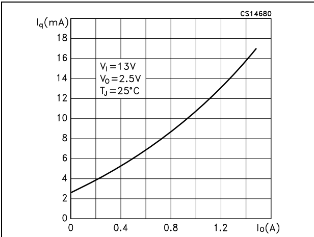
Figure 9. Quiescent current vs. output current ( V_I = 13\text{V} )
