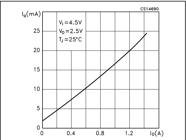
Figure 10. Quiescent current vs. output current ( V_I = 4.5\text{V} )
