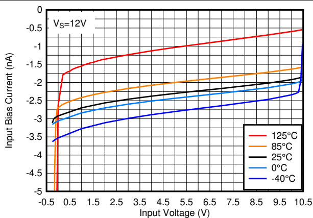
Figure 6-17. Input Bias Current vs. Input Voltage at 12\text{V}
