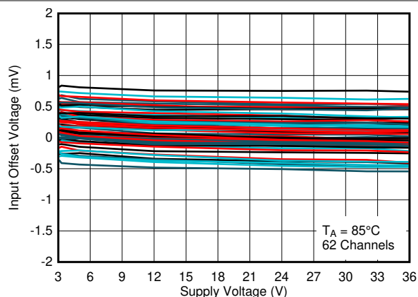
Figure 6-13. Input Offset Voltage vs. Supply Voltage at 85^\circ\text{C}
