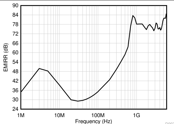
Figure 5-38. EMIRR (Electromagnetic Interference Rejection Ratio) vs Frequency
