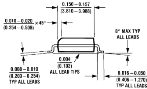
NS Package Number M08A
