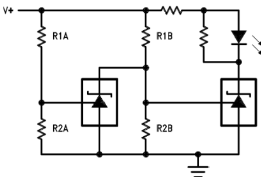
Voltage Monitor
