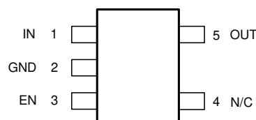
Figure 4-3. DBV Package, 5-Pin SOT-23 (Top View)
