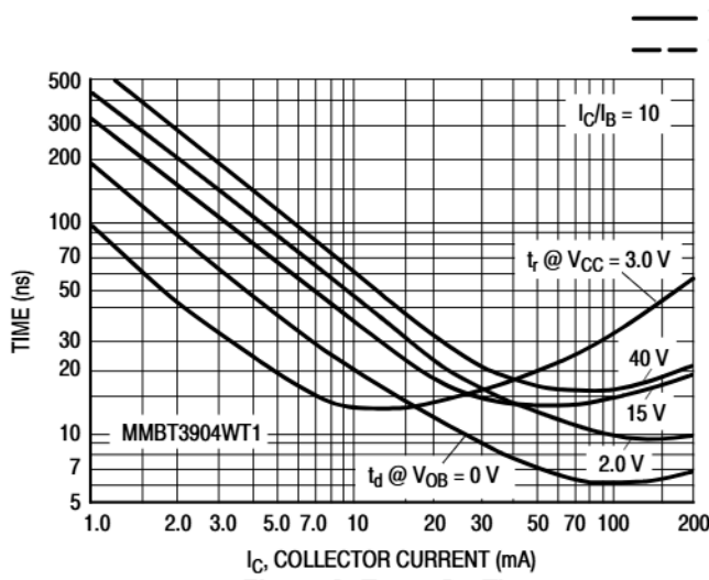
Figure 3. Turn-On Time
