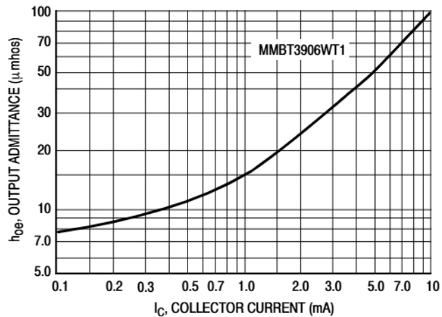
Figure 29. Output Admittance
