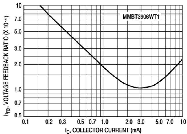
Figure 31. Voltage Feedback Ratio
