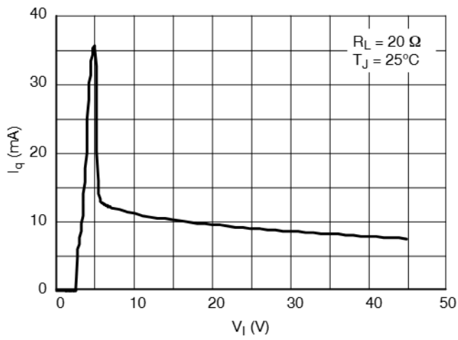
Figure 20. Current Consumption vs. Input Voltage
