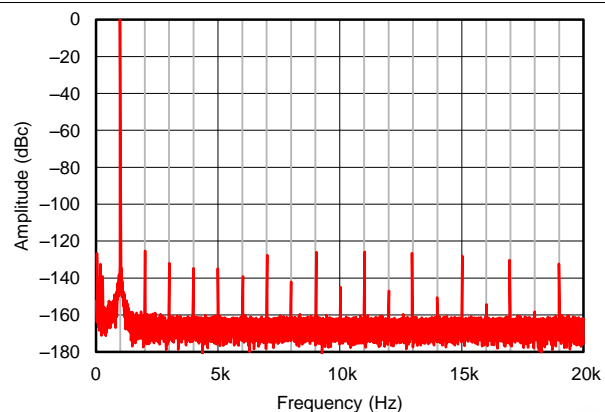
Figure 45. Output Spectrum
