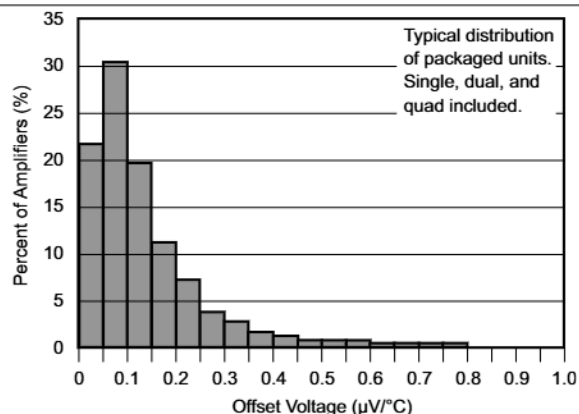
Figure 8. Offset Voltage Drift Production Distribution
