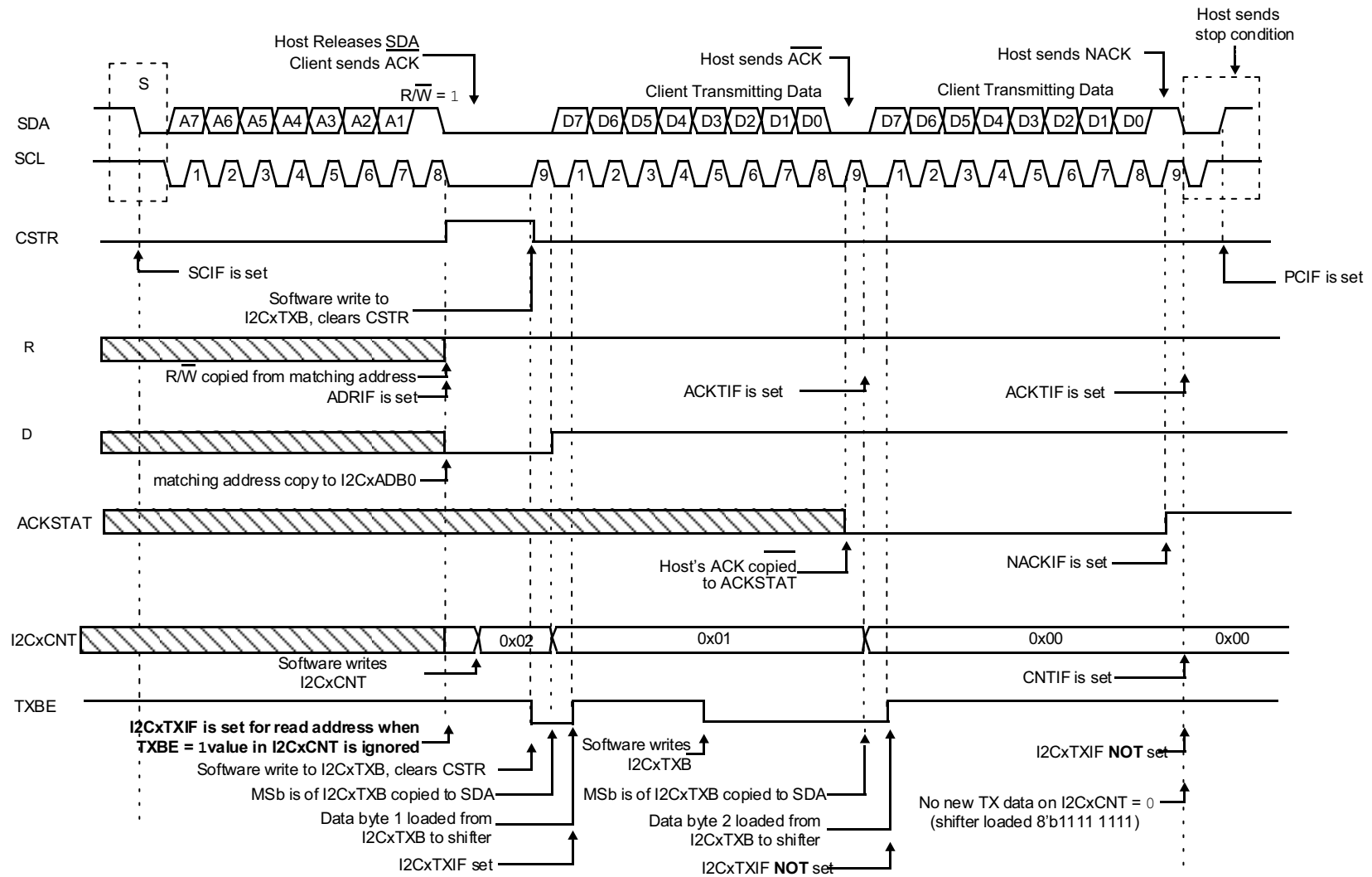
FIGURE 33-9: I 2 C CLIENT, 7-BIT ADDRESS, TRANSMISSION
