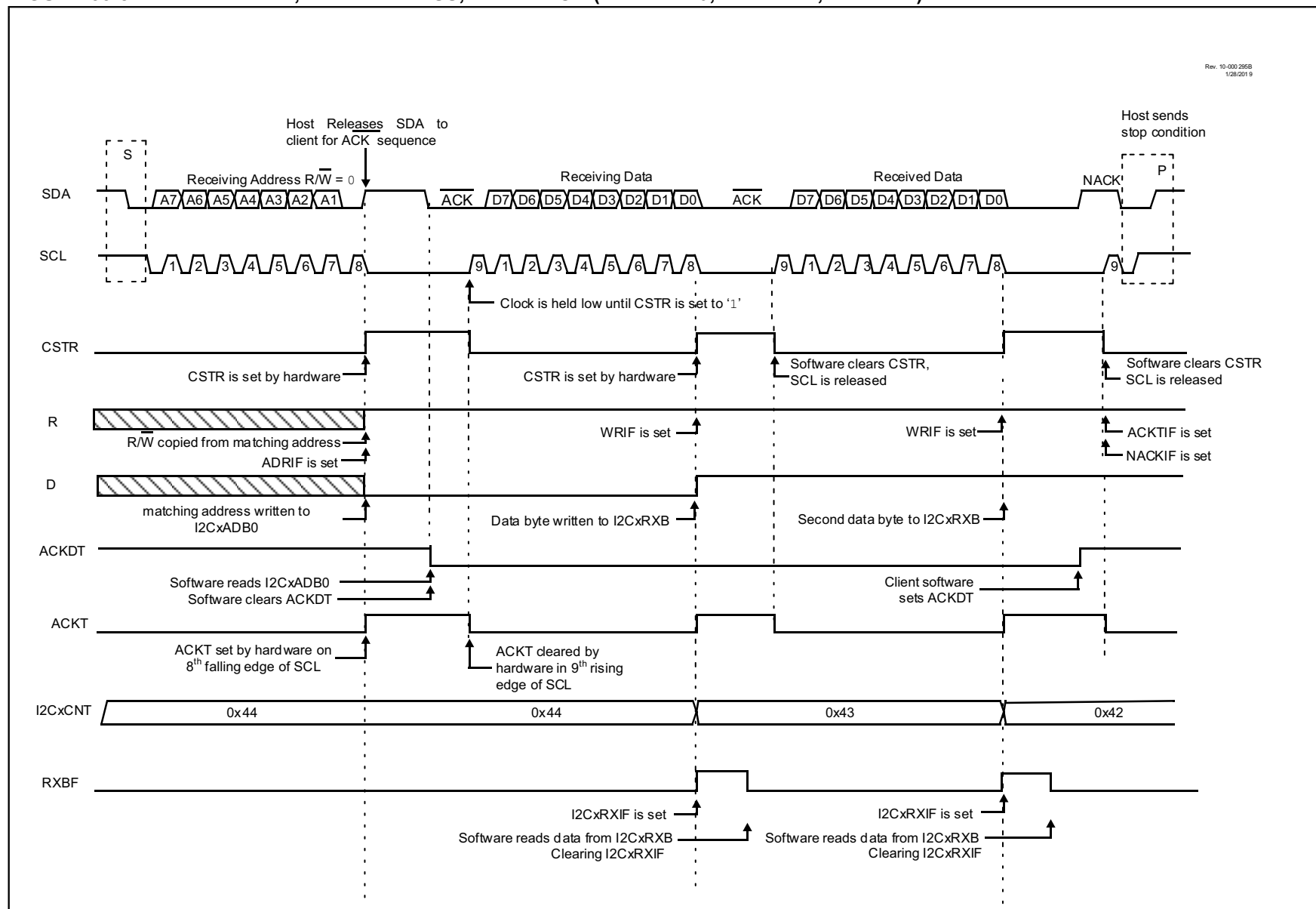
FIGURE 33-8: I 2 C CLIENT, 7-BIT ADDRESS, RECEPTION (ACKTIE = 0, ADRIE = 1, WRIE = 1)
