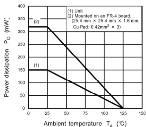
Fig. 7.4 P_D - T_a
