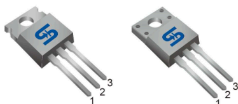
TO-220
